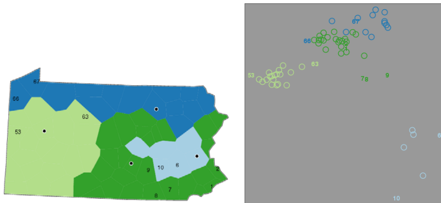
Fig. 9. A novel facility in Gabmap allows researchers to compare the cartographic projection of clusterings (left) with MDS results (right). The MDS plots shows us at glance that the light blue area (around Franklin county) is quite distinct, but also quite diverse, that the southwestern area is nicely distinct, but that the dark green and dark blue areas appear not to be discriminated well, and deserve closer attention. The validation facility allows the user to examine just the two areas in question, a more sensitive view. The numbers on the map (left) re-appear in the MDS plot (right) to enable the researcher to identify sites that do not fit nicely in the clusters.
