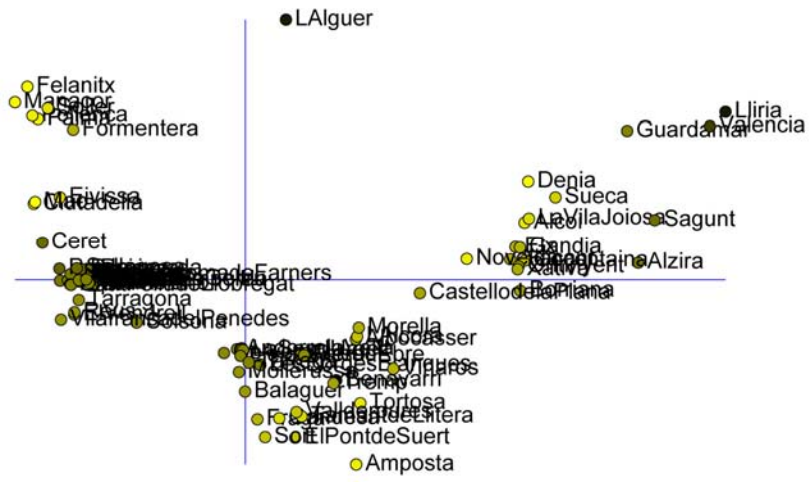
Figure 11 (left) and 12 (right). MDS plot and RGB map obtained using the distance matrix from BCN. R = 0,977
