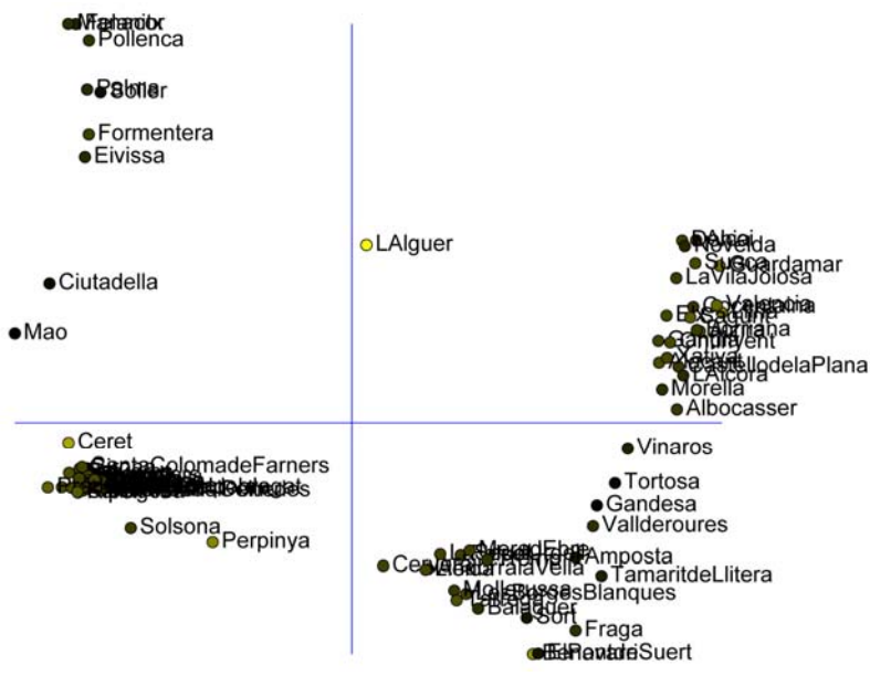
Figure 13 (left) and 14 (right). MDS plot and RGB map obtained using the LD. R = 0,993
