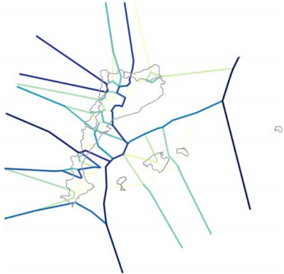
Figure 7. Composite cluster map using the approach from BCN. Number of runs: 100. Amount of noise: 1
