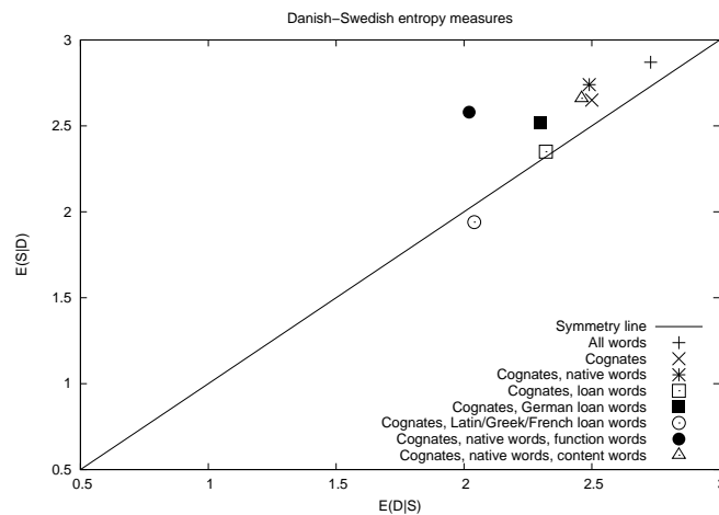
Figure 4: Conditional Entropy between Swedish and Danish, noting Asymmetry
