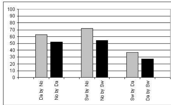
Figure 1: Mean percentage correct answers of three spoken intelligibility tests (Maurud 1976, Bø 1978, Delsing & Åkesson 2005). ‘Da by No’ stands for ‘Percentage correct in Danish test by Norwegians’, etc.
