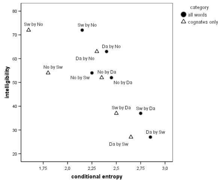
Figure 7: Entropy in Relation to Intelligibility
