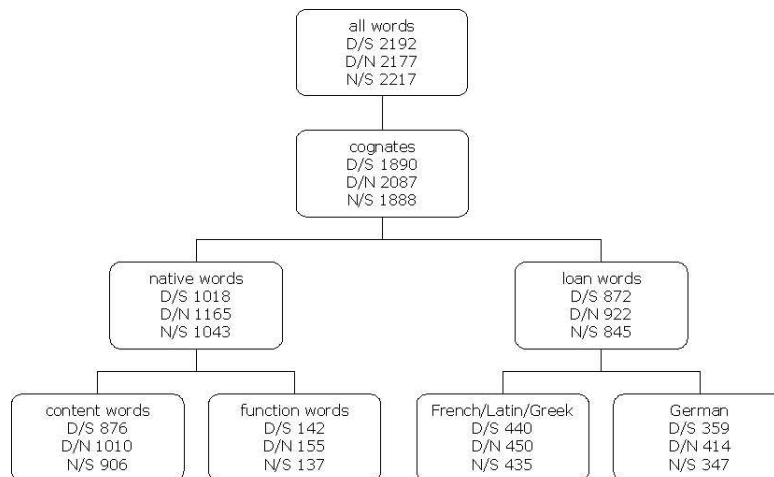
Figure 3: Number of Word Pairs for each of the 8 Categories.
