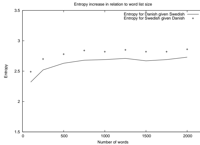
Figure 2: Entropy in relation to word list size
