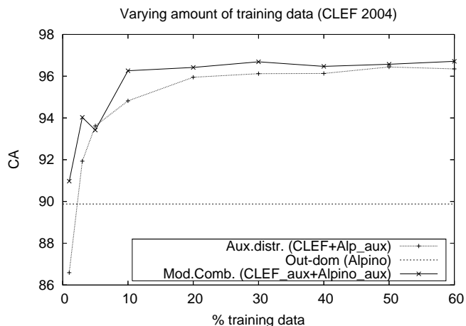
Figure 1: Amount of in-domain training data versus concept accuracy (Similar figures result from the other CLEF datasets) - note that we depict only aux.distr. as its performance is nearly indistinguishable from the in-domain (CLEF) baseline
