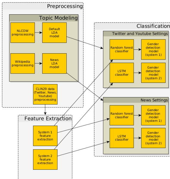
Figure 1: Pipeline overview including both presented systems.
