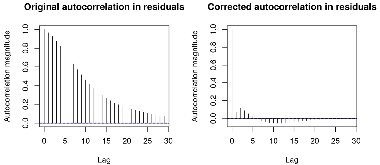
Figure 5. Autocorrelation in the residuals. Left: without correction, right: after correction.
