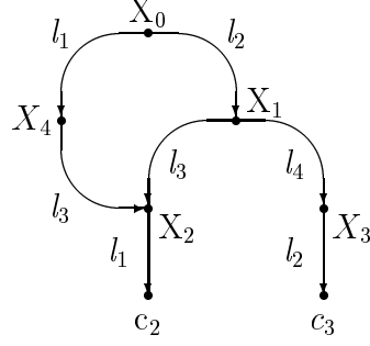
Figure 2.2: The feature graph F_2
