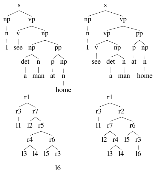
Figure 6: Two parse trees and corresponding derivation trees for I see a man at home
