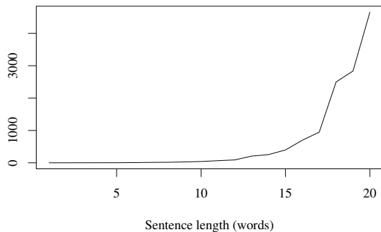
Figure 3: Mean number of parses per sentence length.
