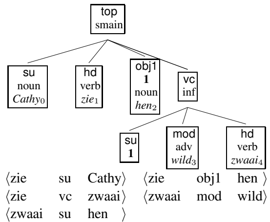
Figure 1: Example of CGN dependency structure for the sentence Cathy zag hen wild zwaaien ( Cathy saw them wave wildly ), with the associated set of dependencies used for evaluation.
