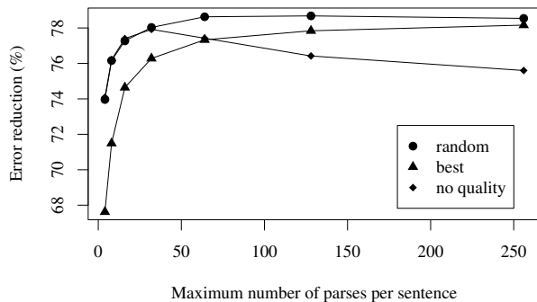
Figure 4: Error reduction versus the maximum number of parses per sentence used for training. Results obtained using ten-fold cross-validation on Alpino treebank.
